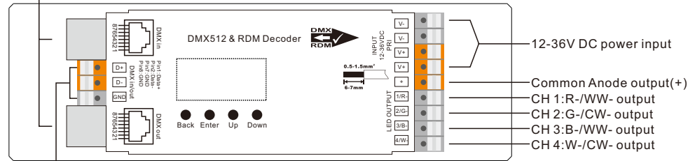
DMX512 input/output
